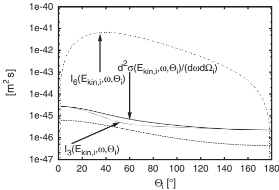
c) E_{kin,i} = 10 MeV, \hbar\omega = 100 keV
