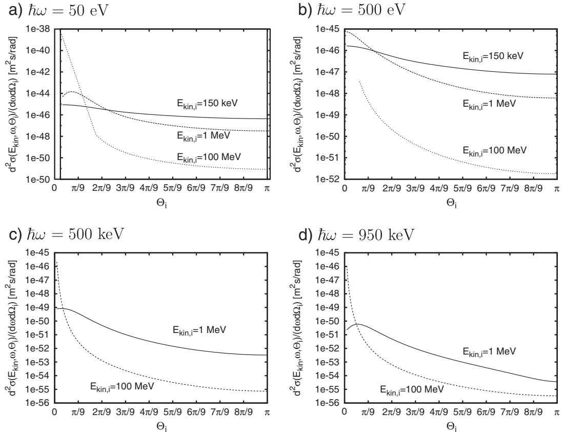
Fig. 8. The doubly differential cross section d^2\sigma/(d\omega d\Omega_i)(E_{kin,i}, \omega, \Theta_i) for Bremsstrahlung ( Z = 7 ) vs. the scattering angle \Theta_i for several electron and photon energies. In each panel the photon energy \hbar\omega is fixed and the cross section is plotted for various kinetic energies of the incident electron.
