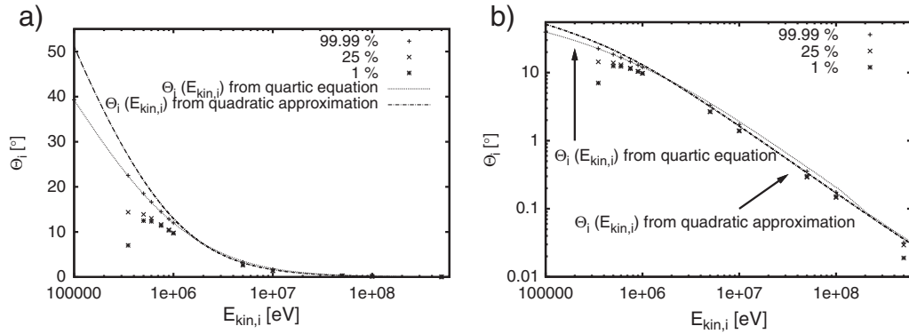
Fig. 9. \Theta_i for maximal scattering vs. incident electron energy in a) semilog and b) log-log plot for Z = 7 . Besides Eq. (114) for \hbar\omega = 0.9999E_{kin,i} the exact solution of the quartic equation and various data for different \hbar\omega/E_{kin,i} are shown.
