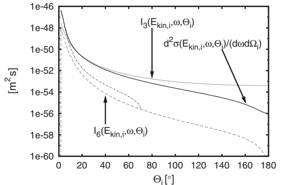
Fig. G.17. Contribution of Eqs. (68)–(73) to Eq. (67) in a semilog plot for different electron and photon energies ( Z = 7 ).
