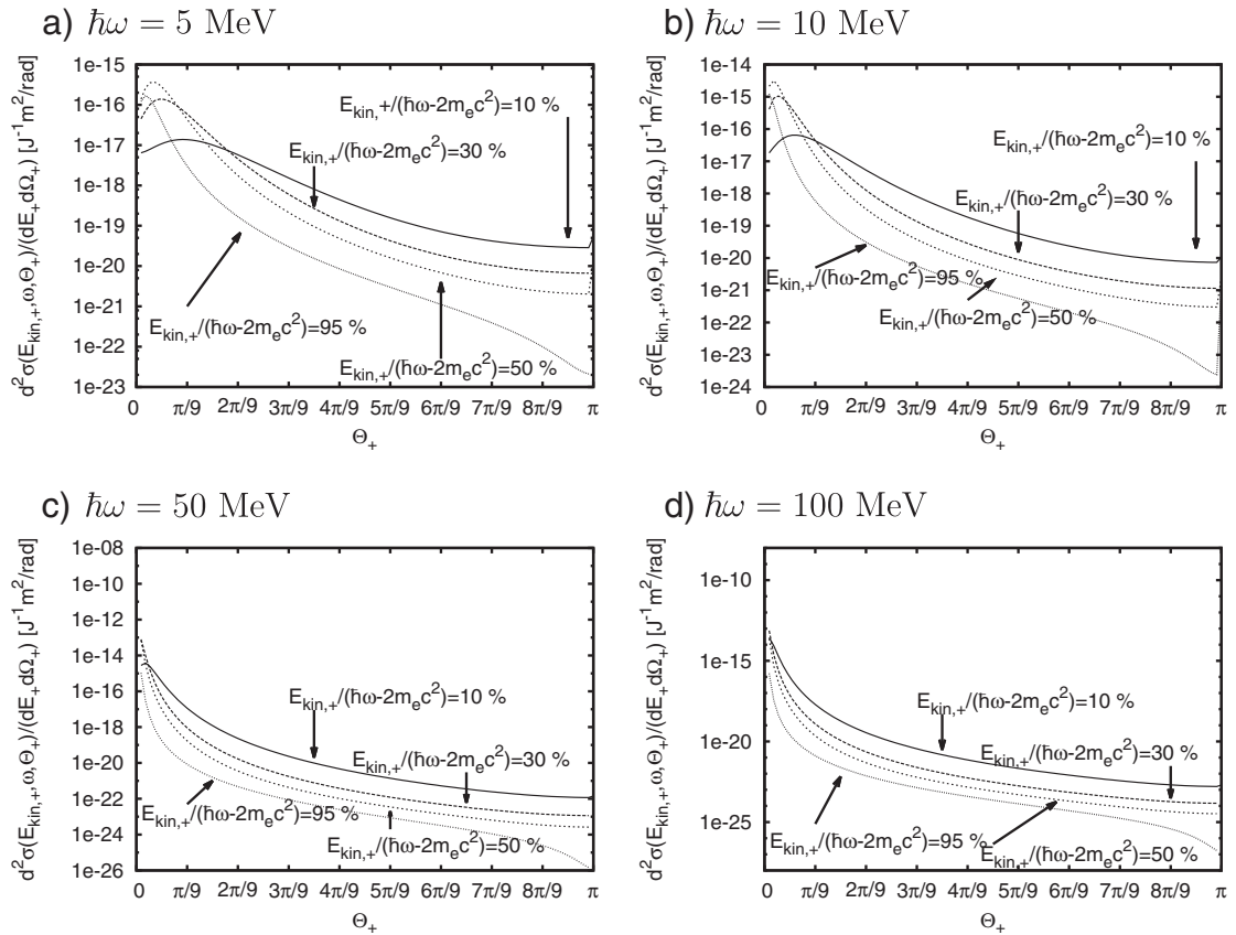
Fig. 10. Doubly differential cross section d^2\sigma(E_+, \omega, \Theta_+)/dE_+ d\Theta_+ for pair production as a function of the angle \Theta_+ between incident photon and created positron for Z = 7 : The cross section is shown for fixed photon energies a) \hbar\omega = 5 MeV, b) \hbar\omega = 10 MeV, c) \hbar\omega = 50 MeV and d) \hbar\omega = 100 MeV. In each panel different positron energies E_+ relative to the available photon energy \hbar\omega - 2m_e c^2 are plotted.
