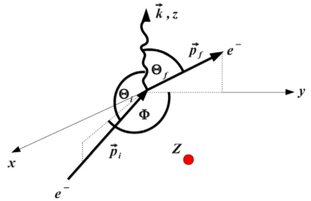
Fig. 1. Parameterization of the Bremsstrahlung process: Momenta of incident electron \vec{p}_i , scattered electron \vec{p}_f and emitted photon \hbar\vec{k} form the angles \Theta_i = \angle(\vec{p}_i, \vec{k}) and \Theta_f = \angle(\vec{p}_f, \vec{k}) , and \Phi is the angle between the planes spanned by the vector pairs (\vec{p}_i, \vec{k}) and (\vec{p}_f, \vec{k}) . The scattering nucleus has atomic number Z .
