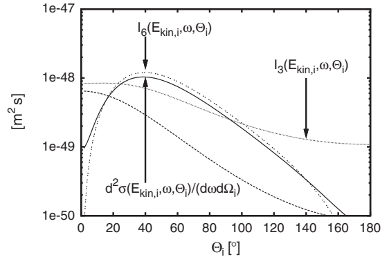
d) E_{kin,i} = 10 MeV, \hbar\omega = 9.5 MeV
